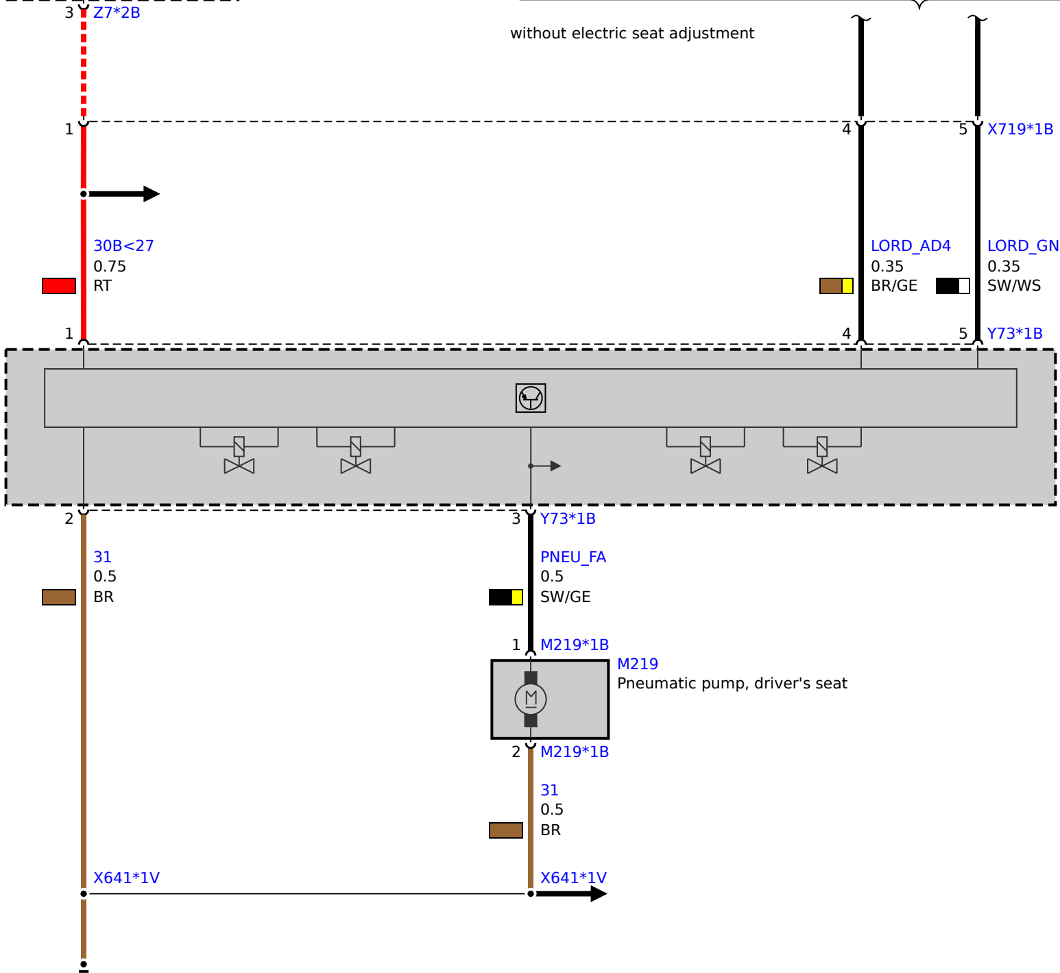
Y73 Valve block, lumbar support, driver
