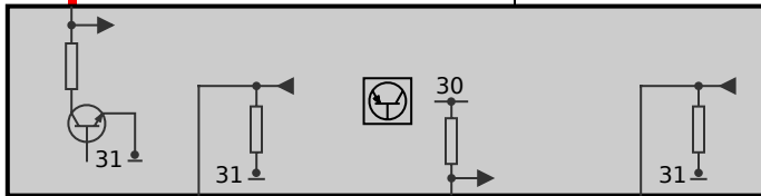
N2 Blower output stage
