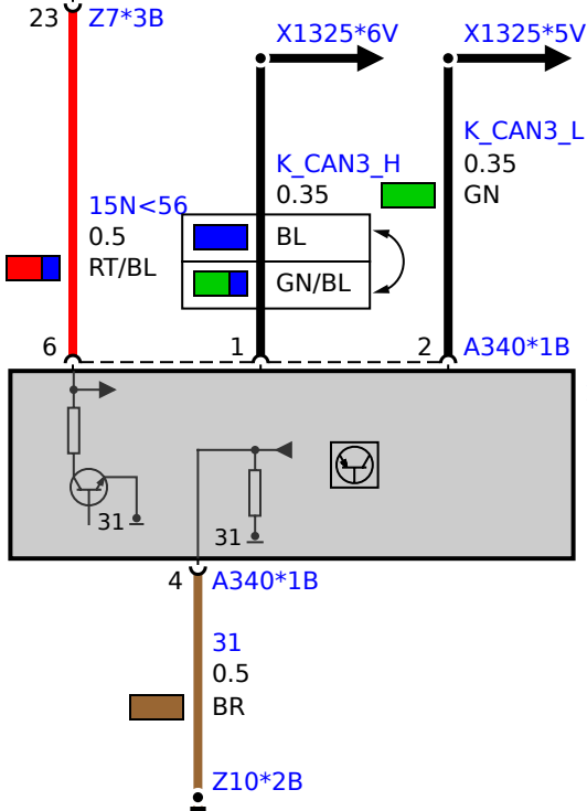
A340 Vehicle Sound Generator
