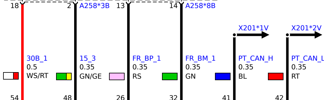
A258 Body Domain Controller
