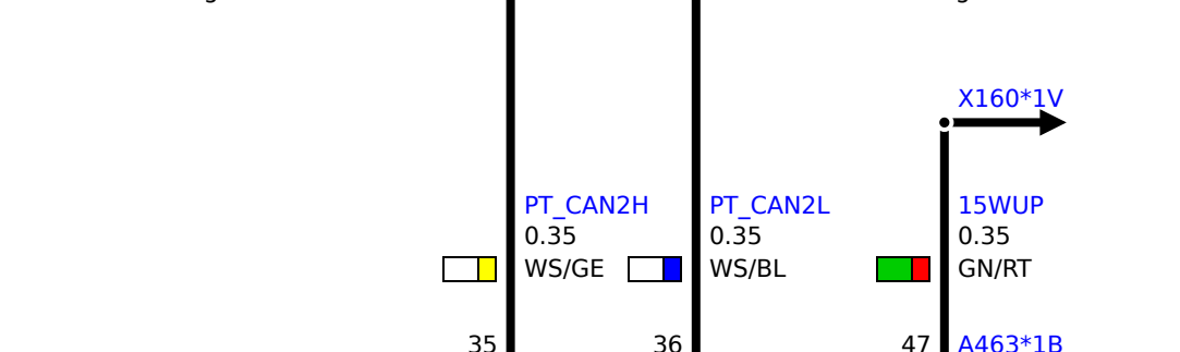
A460 Digital diesel electronics
