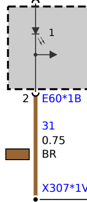
E60 Tail light, inner left 1) Rear fog light
