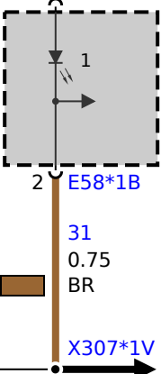
E58 Tail light, inner right 1) Rear fog light
