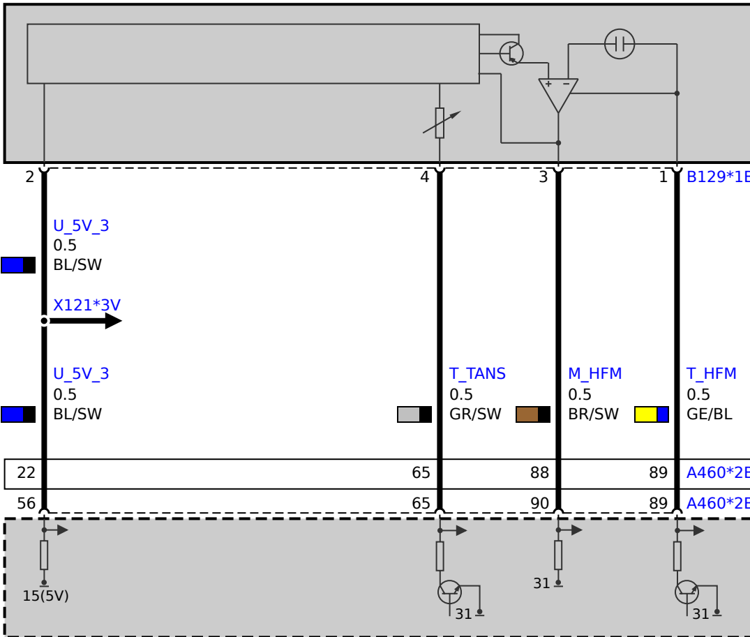
B129 Hot-film air mass meter
