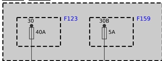
Z2 Fuse holder, rear
