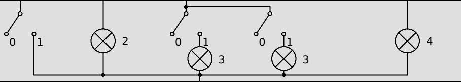
E34 Interior/reading lamp, front 0) OFF 1) ON 2) Interior lamp 3) Reading lamp 4) Top--light
