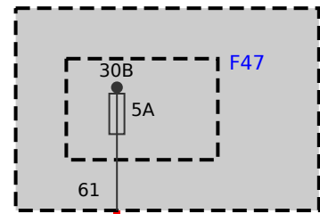
Z44 Front right power distribution box
