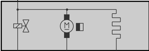
M119a Diagnostic module for fuel tank leakage
