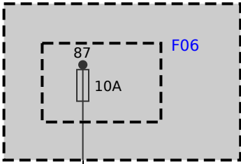
A8681 Fuse carrier, engine electronics
