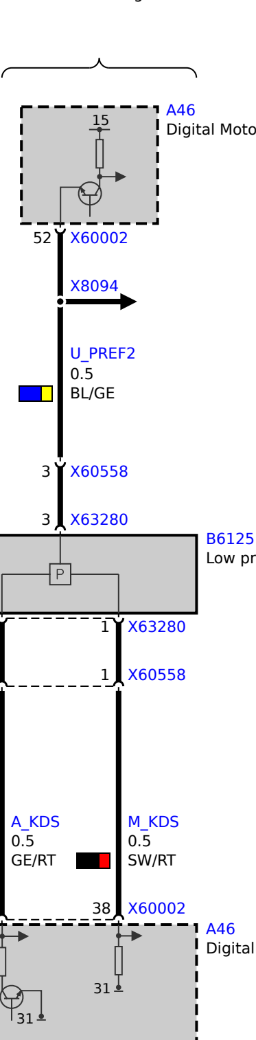
S63 engine
