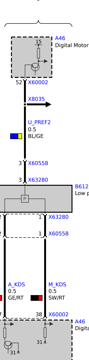
N54 engine
