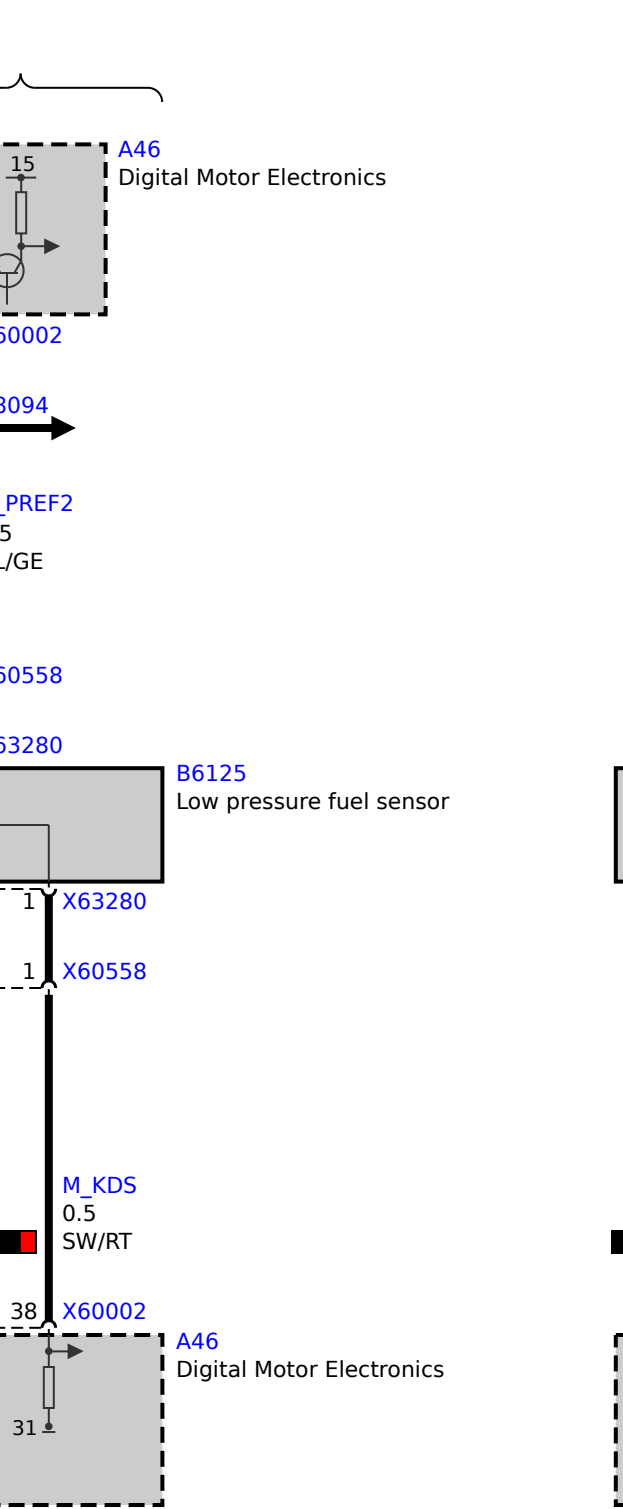
N74 engine
