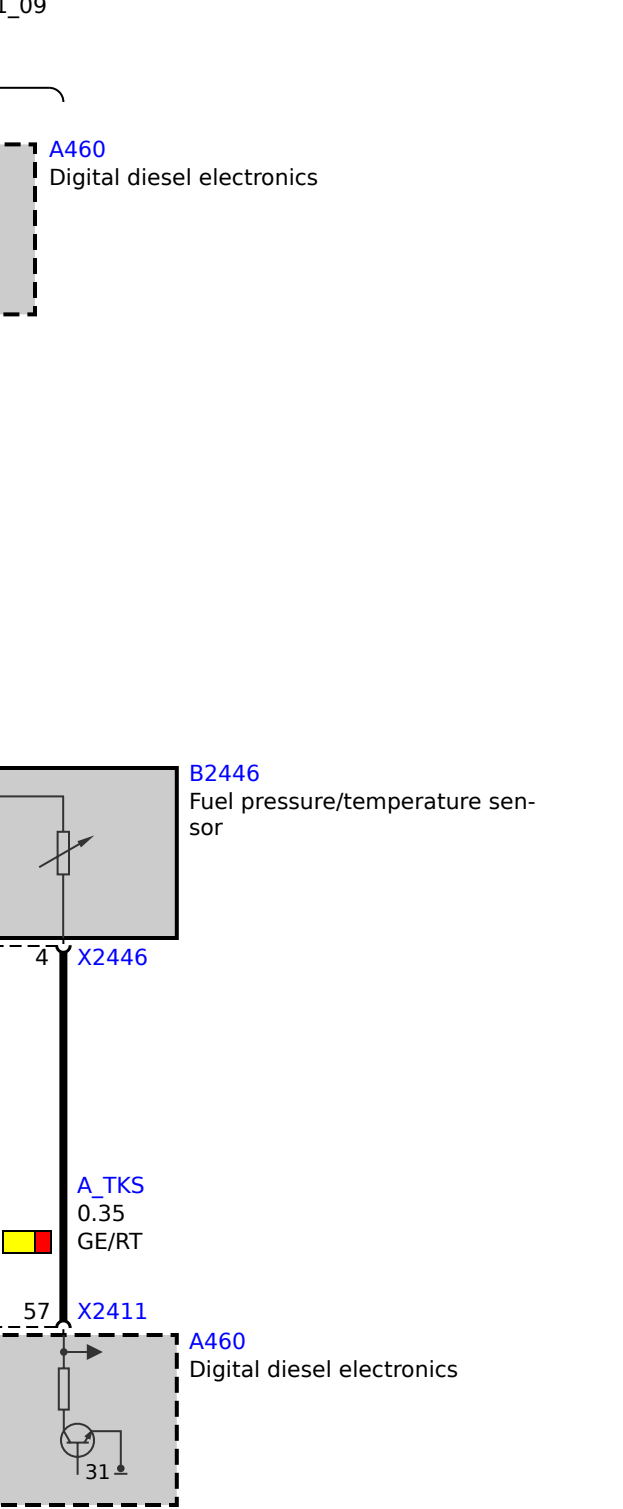
N47 engine without N47 Top after 2011_09
