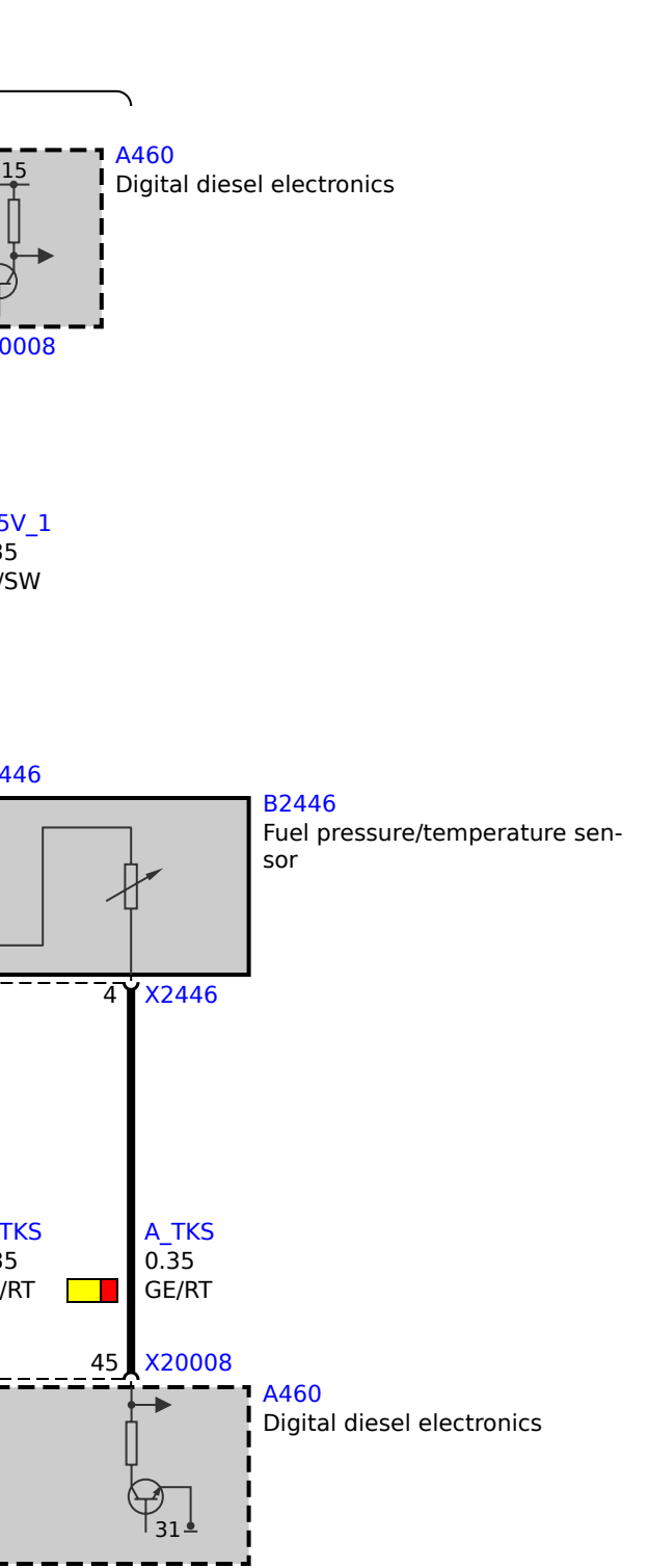
N57 engine
