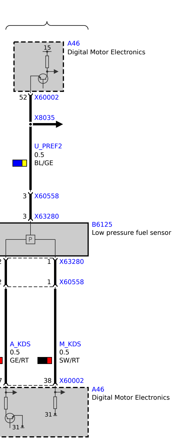
N54 engine
