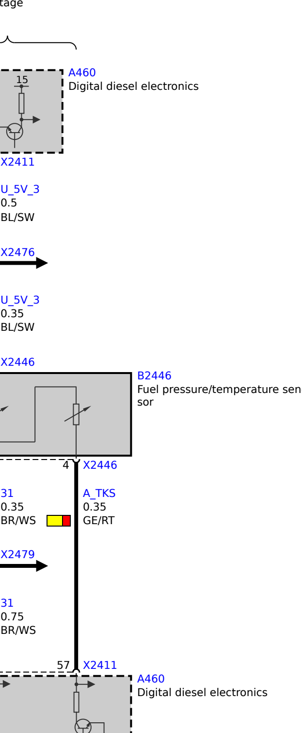
N57TU engine, upper power stage
