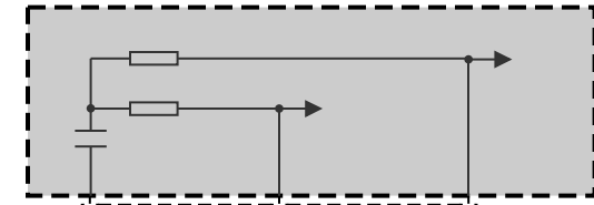
R2a CAN terminator 2
