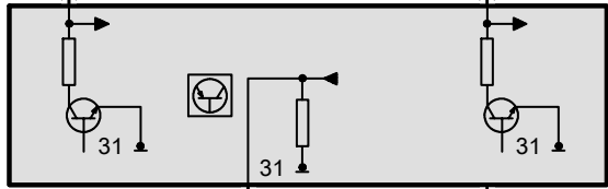
S126 Switch block, driver's door
