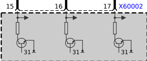
A6000 DME control unit
