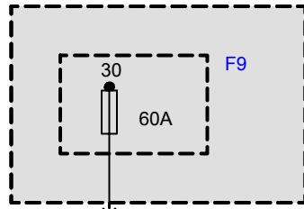
A41a Fuse holder, front
