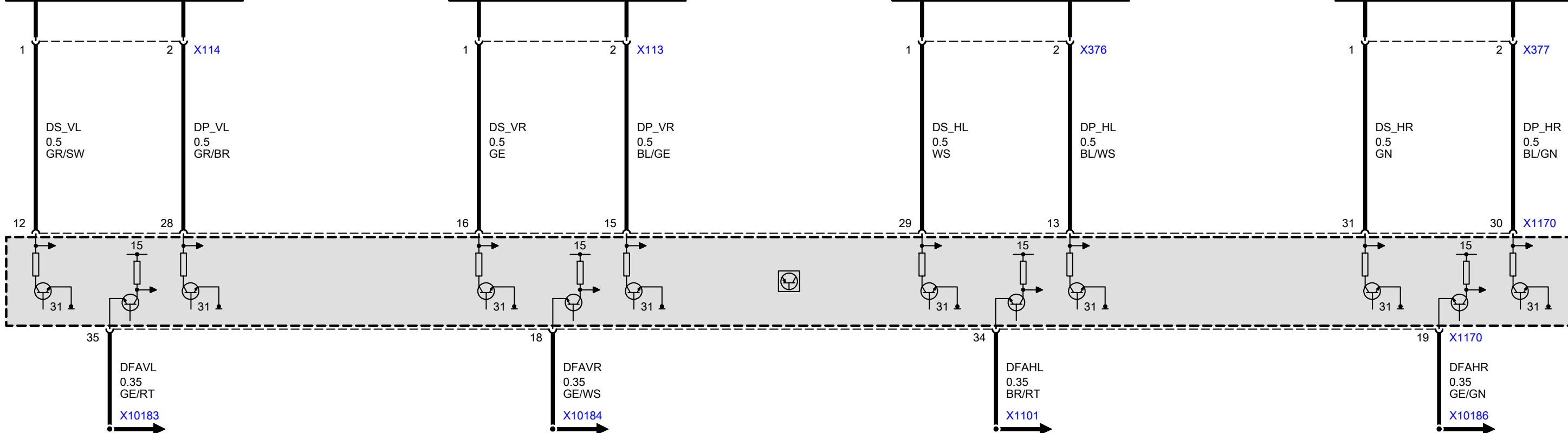
B2 Front left wheel speed sensor
