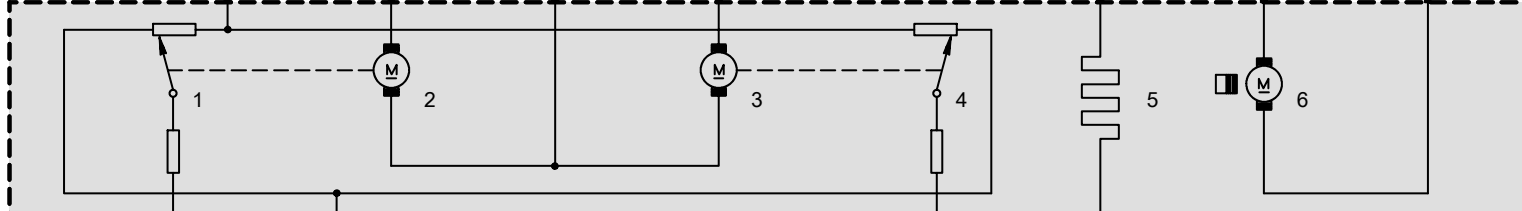
Y5 Outside mirror, driver's side 1) Position potentiometer, vertical 2) Actuator motor, vertical 3) Actuator motor, horizontal 4) Position potentiometer, horizontal 5) Heating 6) Fold--in motor
