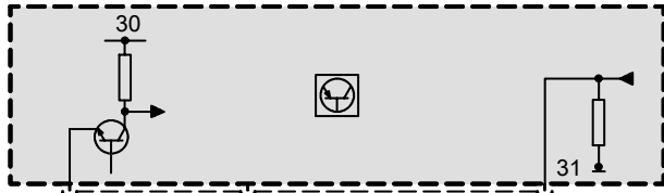
S126 Switch block, driver's door
