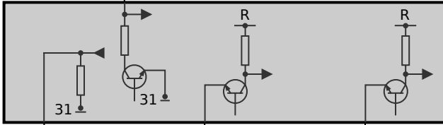
S29 Brake light switch
