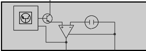
B6207a Hot-film air mass meter
