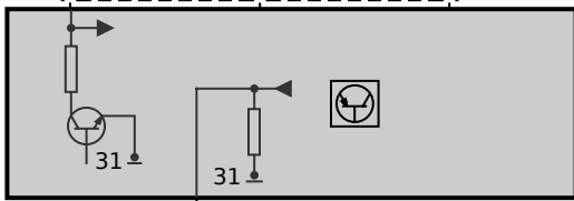
A340 Vehicle Sound Generator
