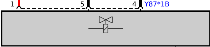
Y87 Valve block, driver's seat backrest width adjustment
