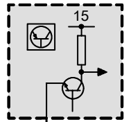
A2a Instrument cluster control unit
