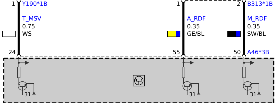
A46 Digital Motor Electronics
