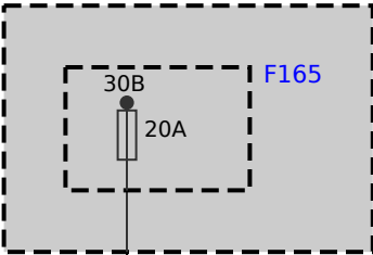
Z2 Fuse carrier, rear
