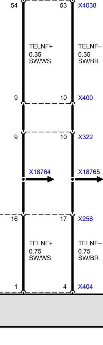
H44 Right front speaker
