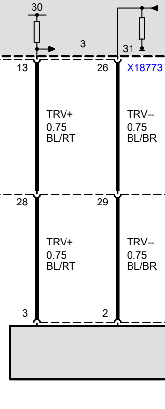
A18 Amplifier 1) Tweeter 2) Mid-range speaker 3) Woofer
