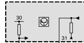
U407 Basic interface, telephone
