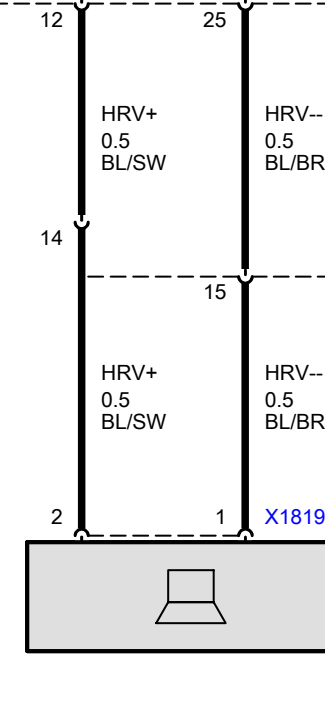
H50 Right front high range speaker
