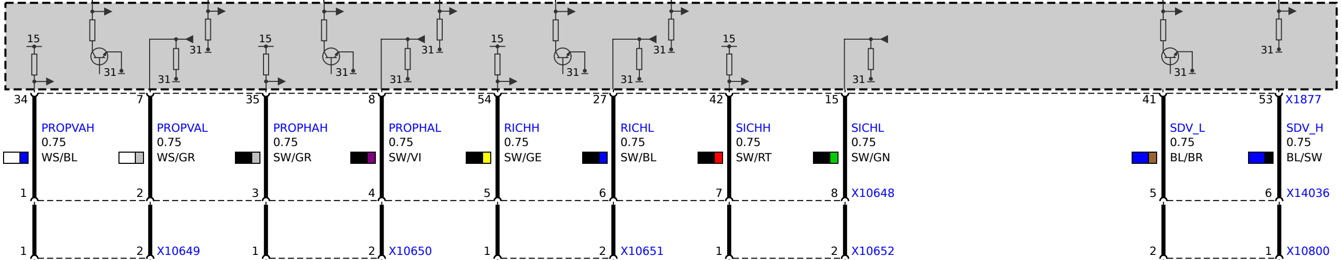
Y40 Valve block dynamic drive 4) Proportional valve, front axle 5) Proportional valve, rear axle 6) Directional control valve 7) Fail-safe valve
