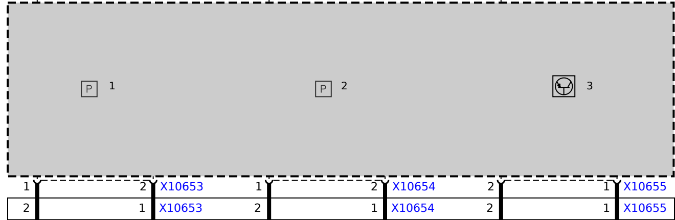
Y40 Valve block dynamic drive 1) Pressure sensor, front axle 2) Pressure sensor, rear axle 3) Switch position detection sensor
