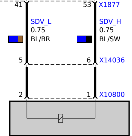
Y40 Valve block dynamic drive 4) Proportional valve, front axle 5) Proportional valve, rear axle 6) Directional control valve 7) Fail-safe valve
