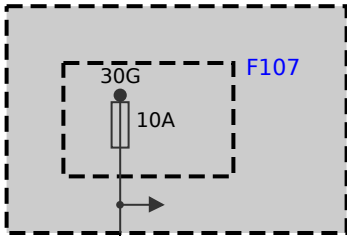
A42 Rear power distribution box
