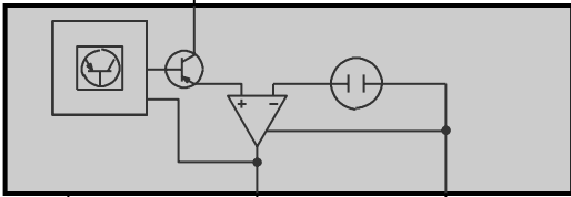
B6207a Hot-film air mass meter
