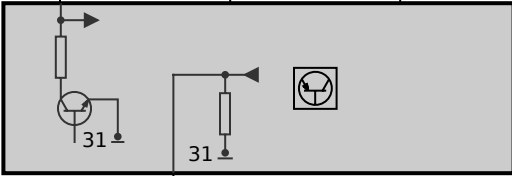
A340 Vehicle Sound Generator
