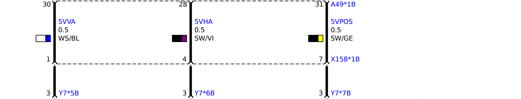
Y7 Valve block, dynamic drive 1) Pressure sensor, front axle 2) Pressure sensor, rear axle 3) Shift position sensor
