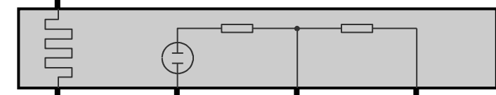
B62101 Oxygen sensor before catalytic converter
