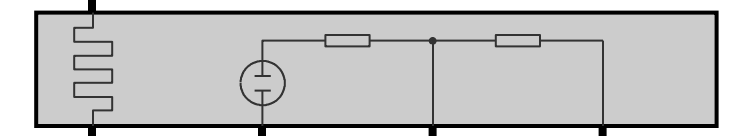
B62201 Oxygen sensor 2 before catalytic converter
