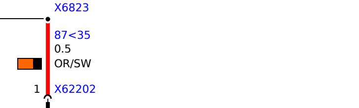
B62102 Oxygen sensor after catalytic converter
