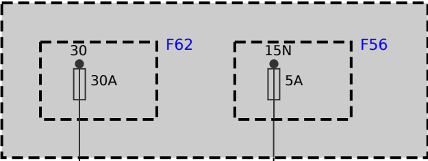
Z7 Front power distribution box
