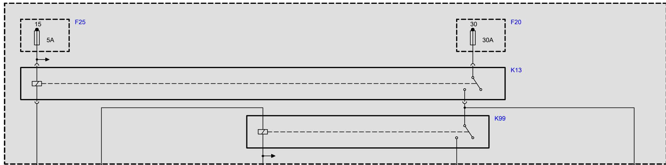
A41 Power distribution
