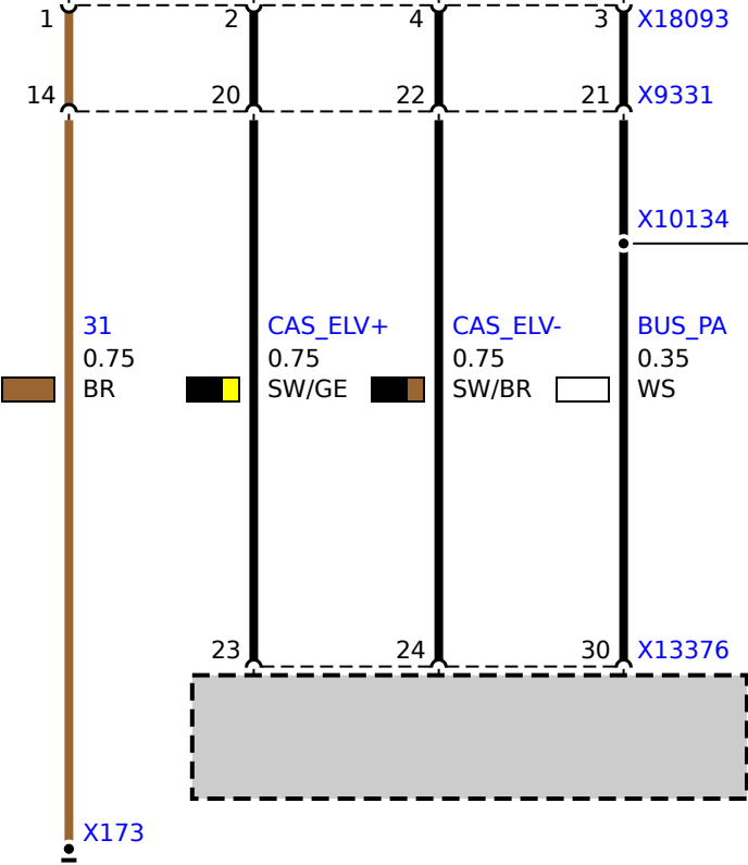
A149a Car access system
