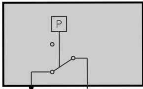
B6231 Oil pressure switch
