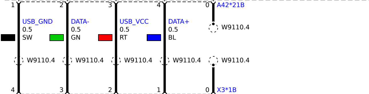
X3a USB port
