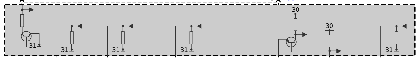
A604 Control electronics for armrest heating of front centre console
