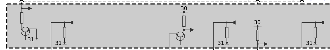
A514 Door control unit, passenger door (TSGBF)
