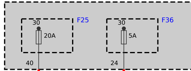
Z44 Front right power distribution box
