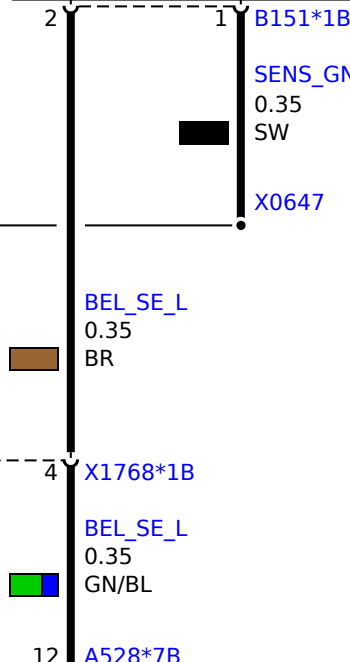
A528 Basic central platform (BCP)
