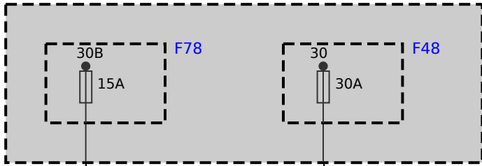
Z7 Front power distribution box
