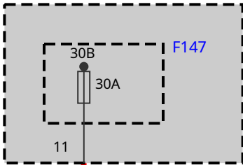
Z43 Front left power distribution box
