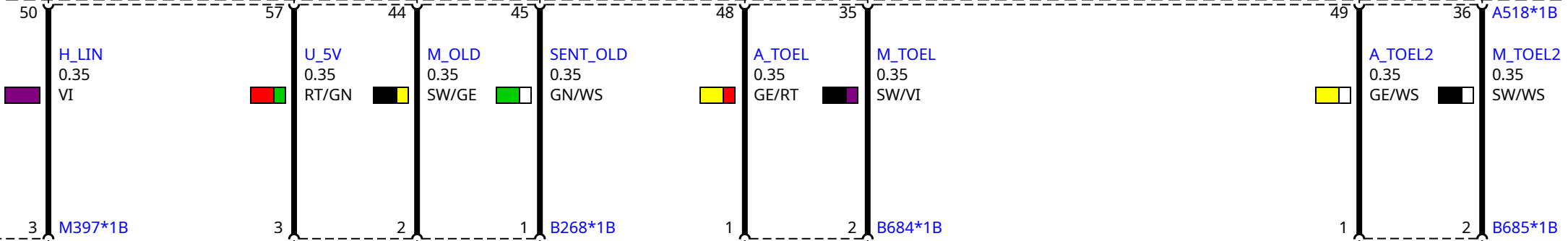
I03 Oil module 1) Electric oil pump 2) Oil pressure sensor 3) Oil temperature sensor
