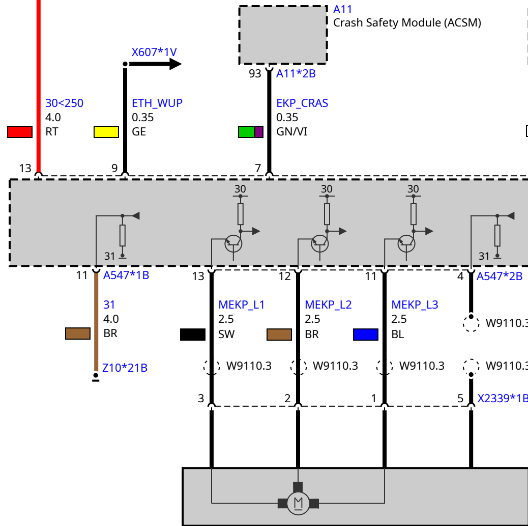
A11 Crash Safety Module (ACSM)
