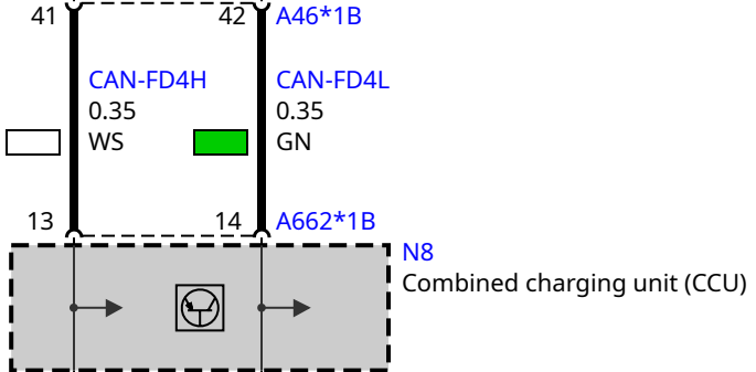
N8 Combined charging unit (CCU)
