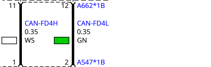
A547 Tank function electronics (TFE)
