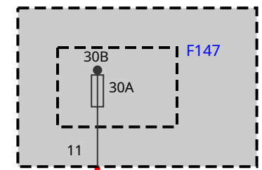
Z43 Front left power distribution box
